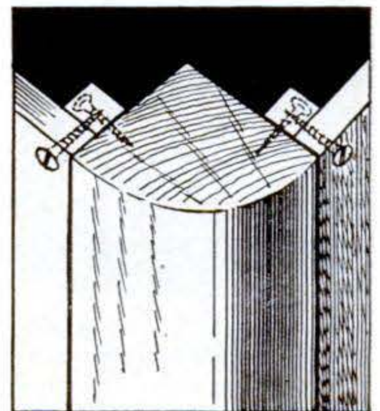
ROUNDING BY HAND: Plane corner to 45°, reduce high spots of angle by more planing, and finish by hand. Built-up corner is at right.
